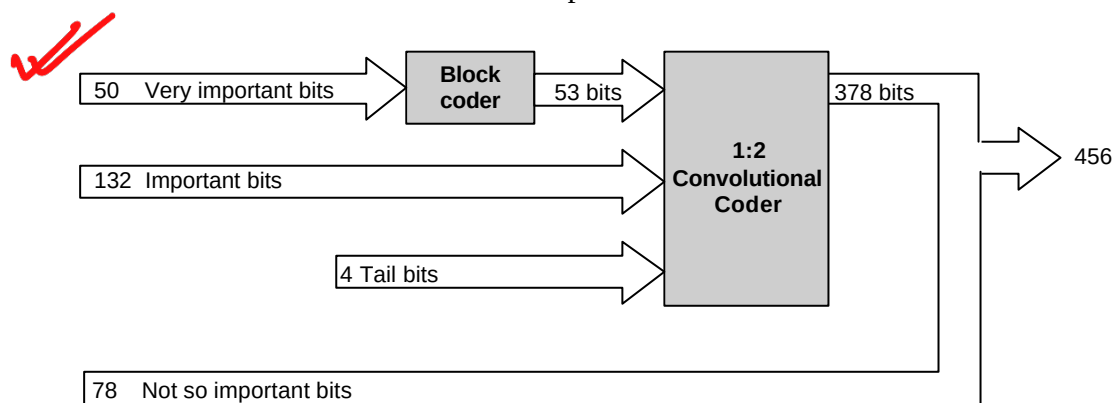
Figure 3-28 Channel coding
