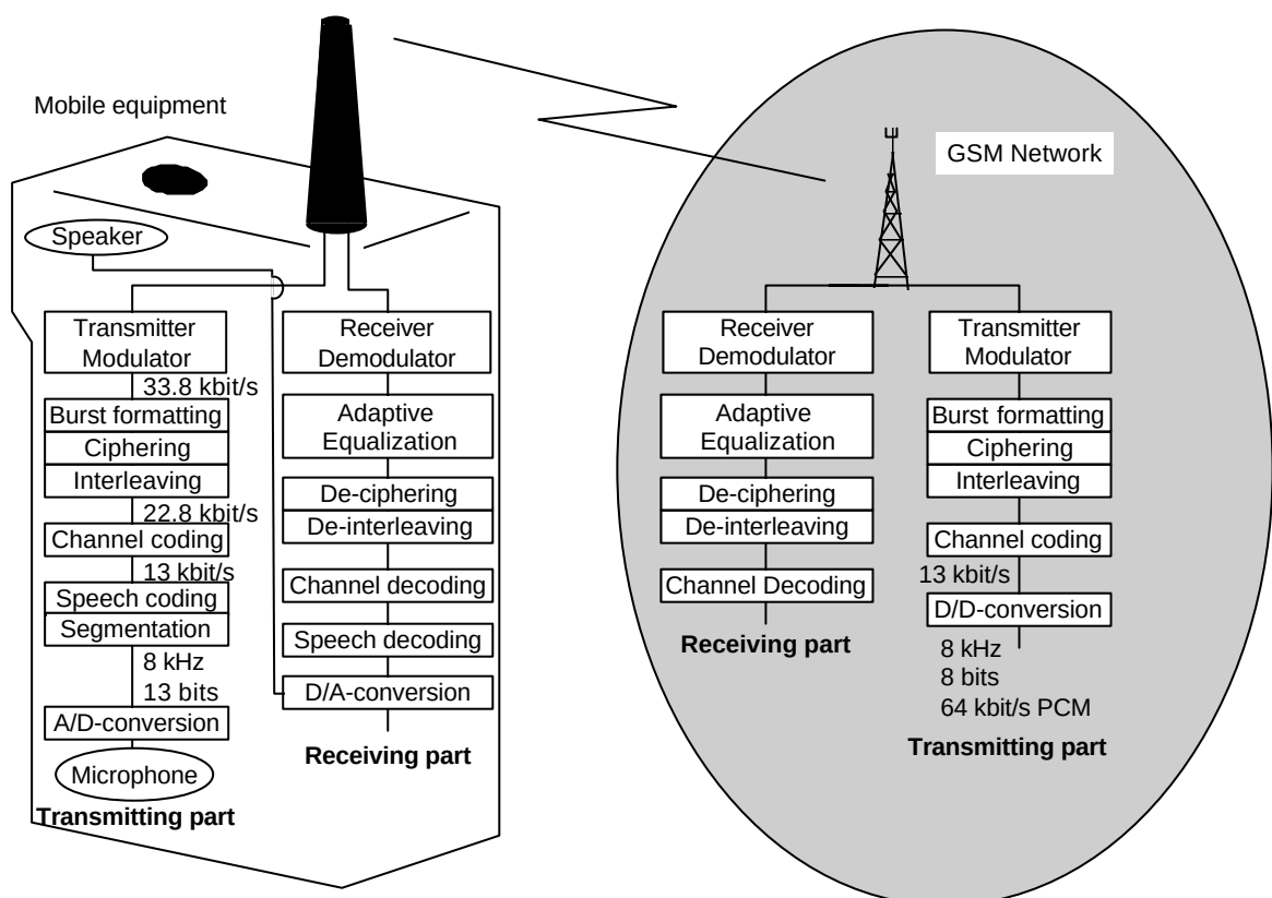
Figure 3-33 GSM transmission process
