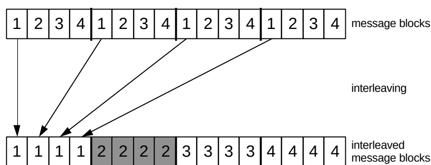
Figure 3-17 Interleaving
