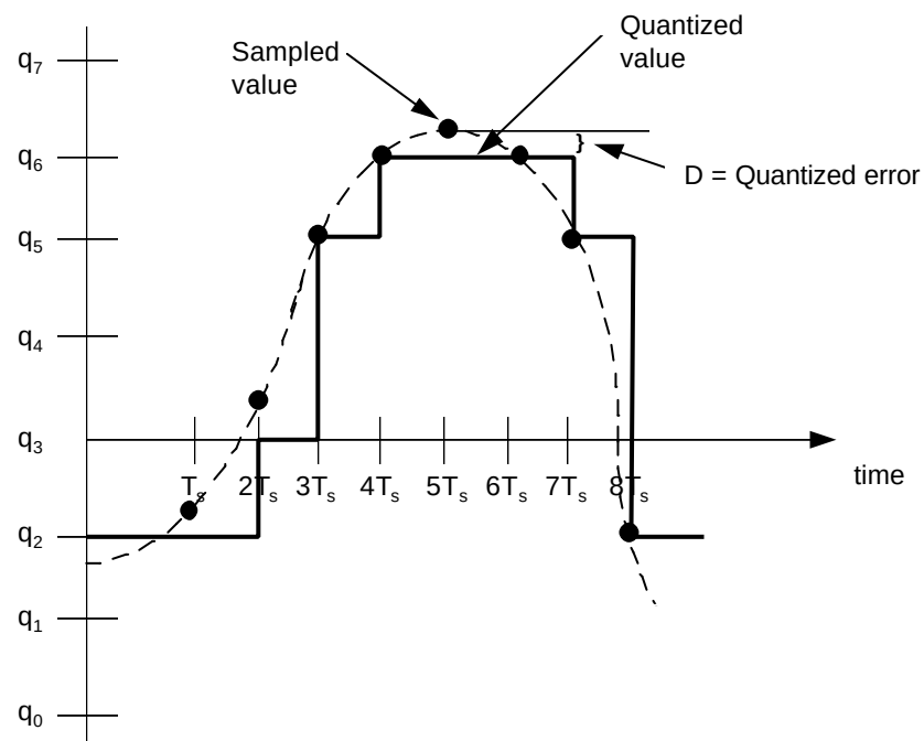
Figure 3-25 Quantization
