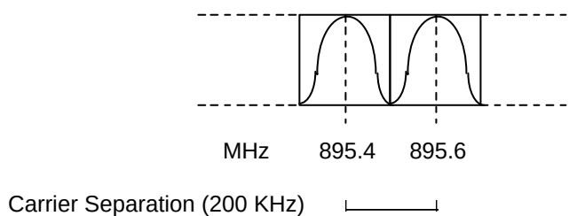
Figure 3-5 Carrier separation
